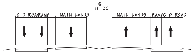
TYPICAL SECTION @ STATIONS 496+02 & 497+43 NT6
