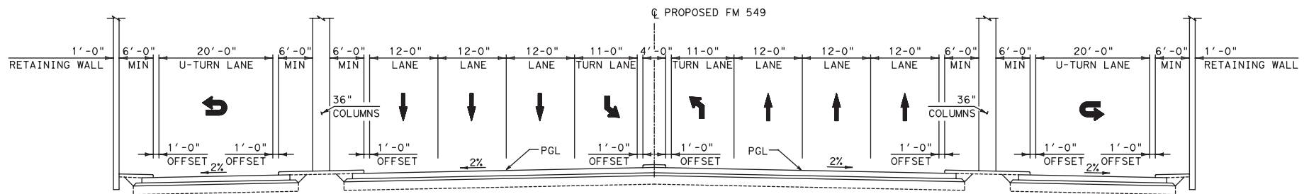
PROPOSED FM 549 ROADWAY SECTION
